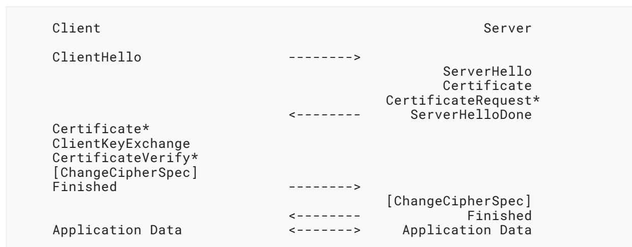
Figure 1: Message Flow for a Full Handshake
