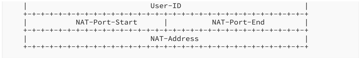
Figure 58: Subscriber CGN Port Range TLV
