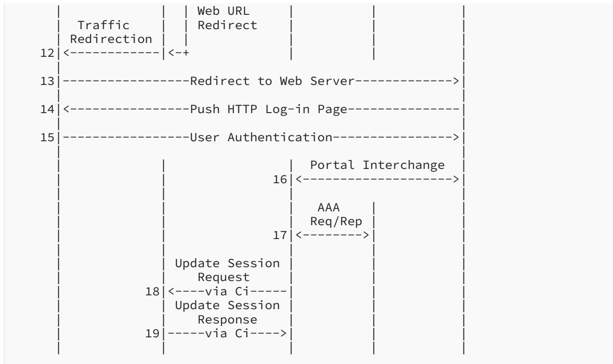
Figure 23: WLAN Access
