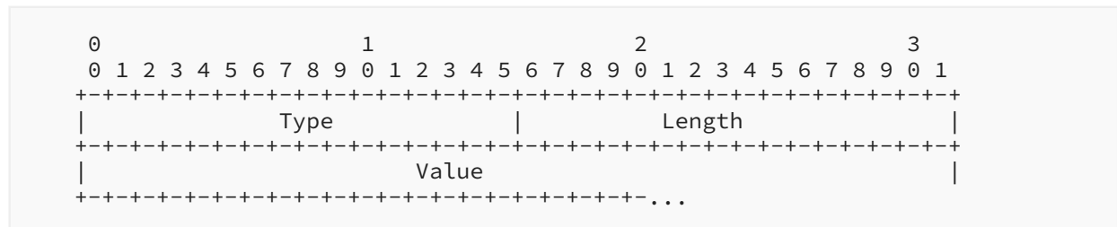
Figure 33: Sub-TLV Header
