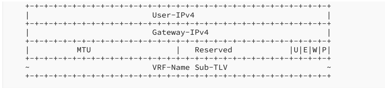
Figure 48: IPv4 Subscriber TLV
