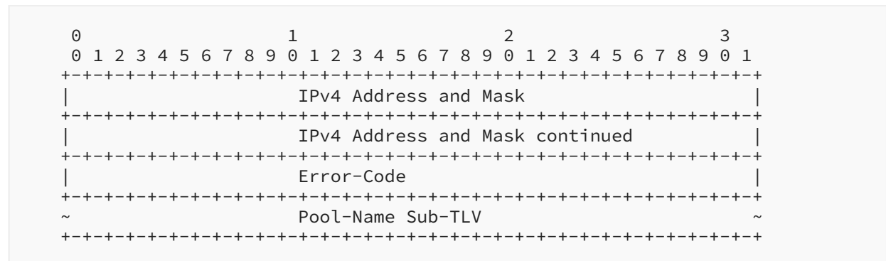
Figure 64: Address Renewal Response TLV
