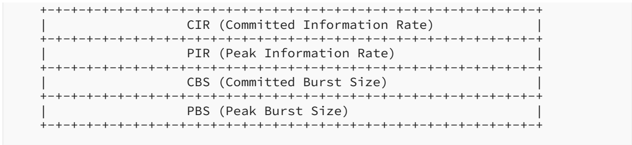
Figure 35: Egress-CAR Sub-TLV
