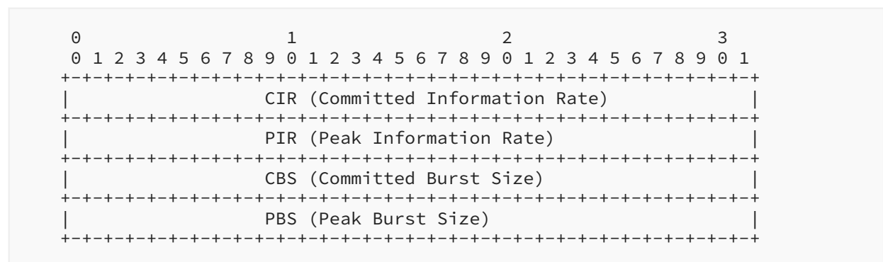
Figure 34: Ingress-CAR Sub-TLV
