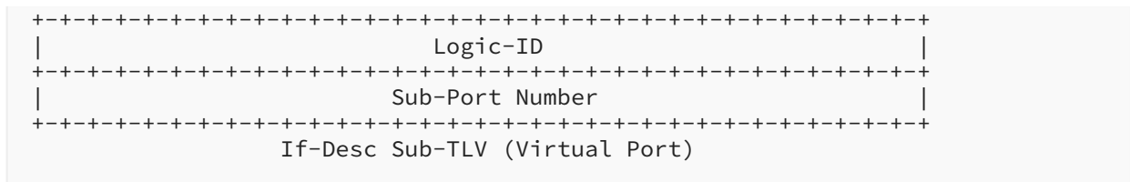
Figure 36: If-Desc Sub-TLV Formats
