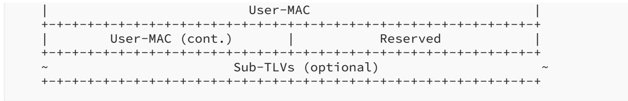
Figure 51: IPv6 Static Subscriber Detect TLV
