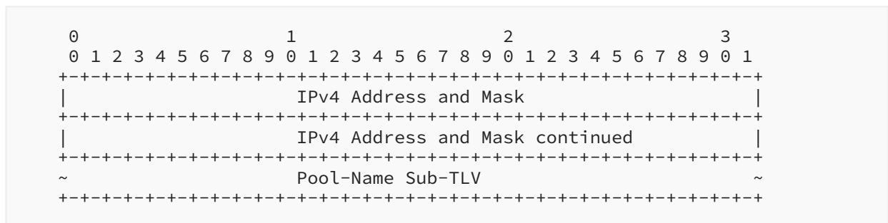
Figure 63: Address Renewal Request TLV
