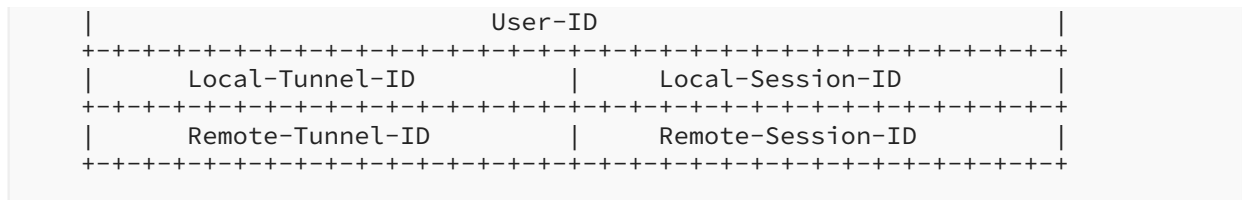
Figure 52: L2TP-LAC Subscriber TLV
