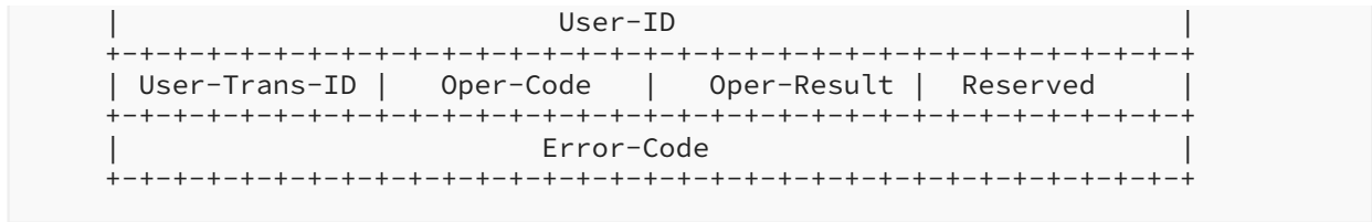
Figure 56: Update Response TLV
