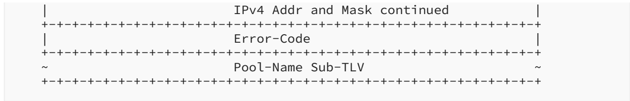
Figure 62: Address Assignment Response TLV
