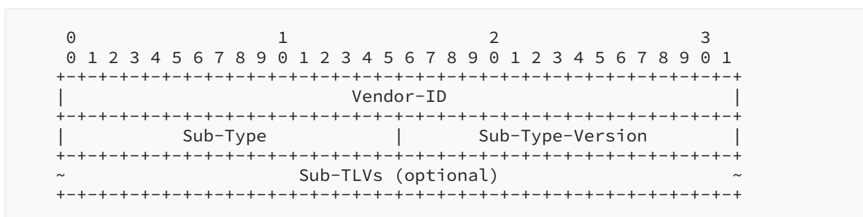
Figure 69: Vendor TLV
