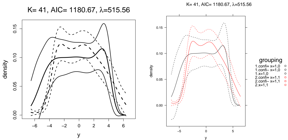
Figure 5: Plot of the estimated densities of Allianz in 2006 and 2007.
